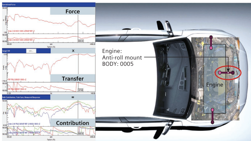
Figure 5: Anti-roll mount identified as most dominant path at 3,800 RPM.
