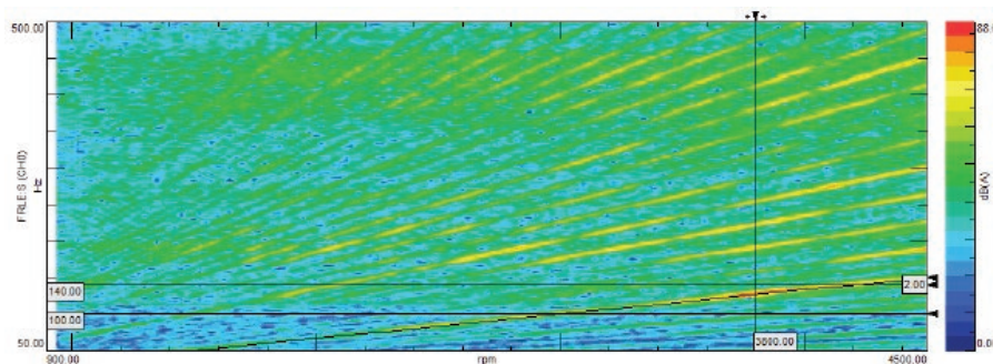
Figure 3: Top: Sensor locations. Bottom: Color map of a vehicle showing low-frequency booming noise.
